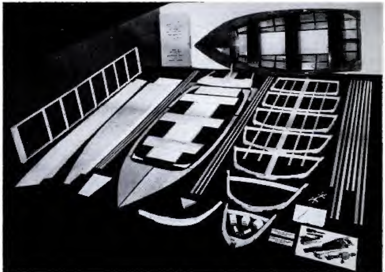
Except for the hand tools, here's what you get with the typical boat kit. Completed boat is in the background
